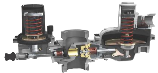
Typical CSB404 Regulator with Slam-shut Internal View
